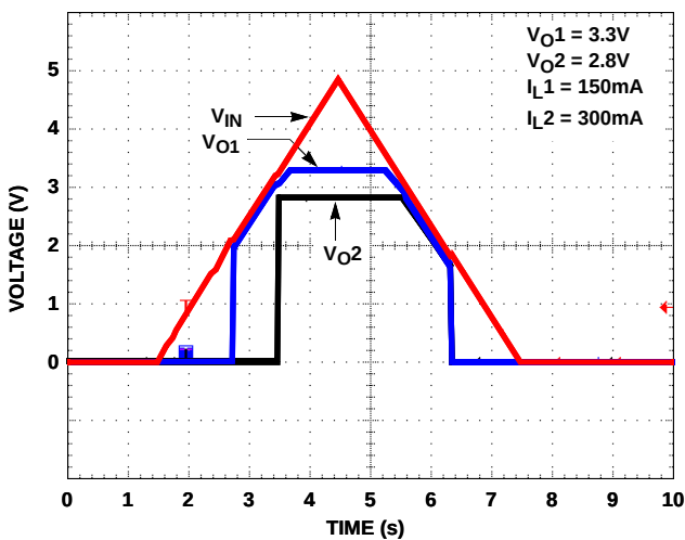
FIGURE 11. POWER-UP/POWER-DOWN
