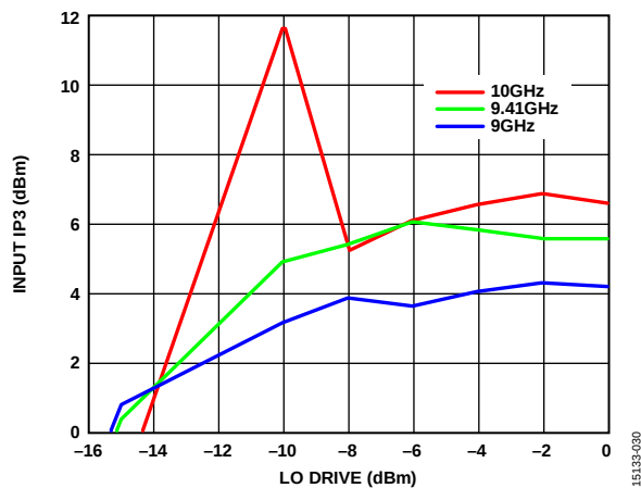
Figure 30. Input Third-Order Intercept (IP3) vs. LO Drive at Various RF Frequencies
