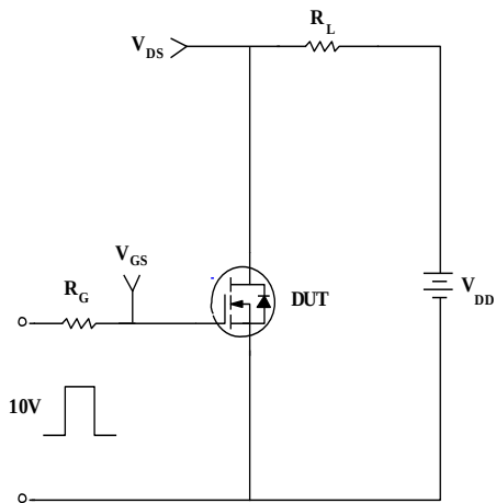
2) Resistive Switching Test Circuit & Waveforms
