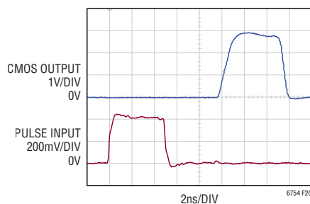
Figure 20. Pulse Input and Output
