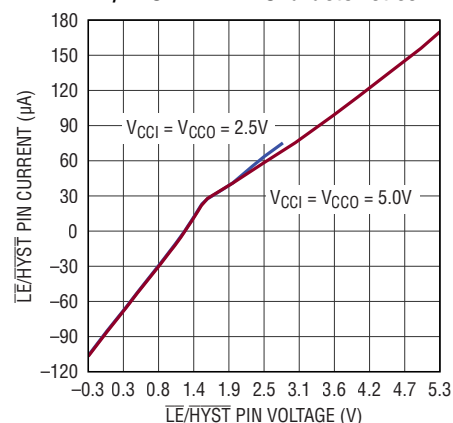
LE/HYST Pin I-V Characteristics
