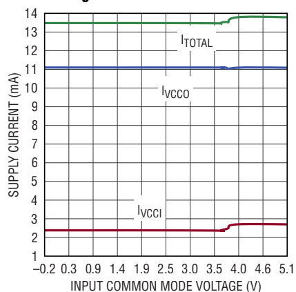
Supply Current vs Common Mode Voltage
