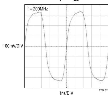
Differential Output Toggle Waveform
