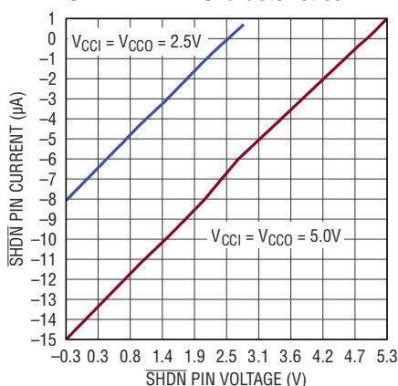
SHDN Pin I-V Characteristics
