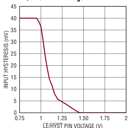
Input Hysteresis vs LE/HYST Pin Voltage
