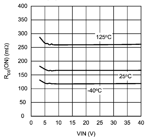
R_{DS(ON)} vs V_{IN} @ I_{SW} = 1A
