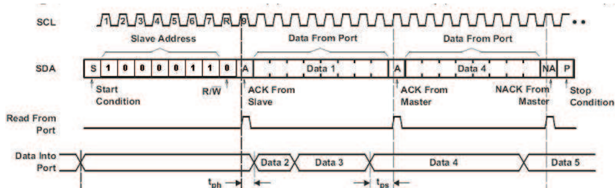
Figure 7. Read From Input Status Register
