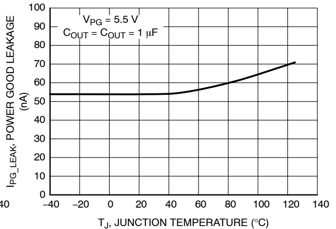
Figure 74. PG Pin Leakage vs. Temperature
