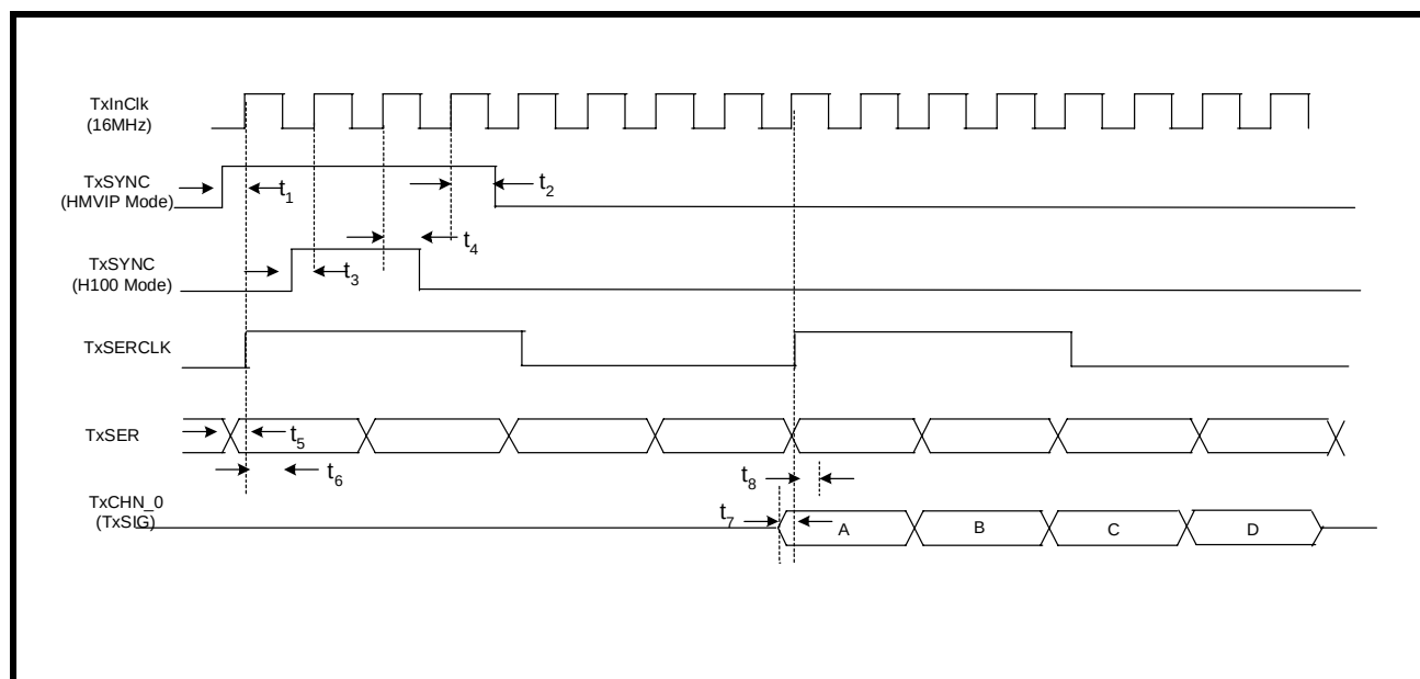
FIGURE 5. FRAMER SYSTEM TRANSMIT TIMING DIAGRAM (HMPVP AND H100 MODE)
