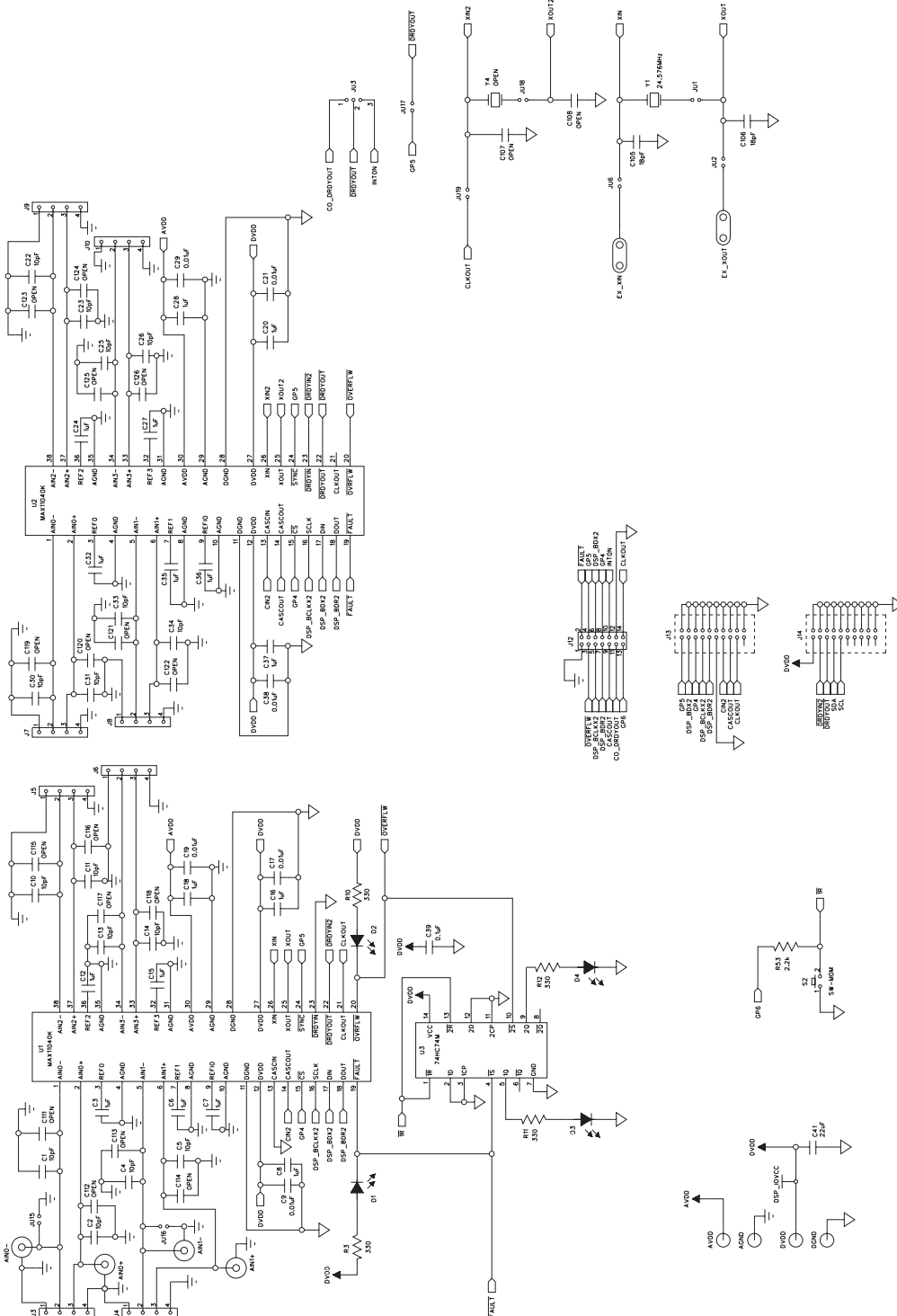
Figure 2a. MAX11040K EV Kit Schematic (Sheet 1 of 4)
