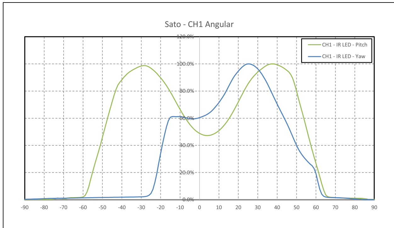
Figure 15: Typical Proximity Angular Response
