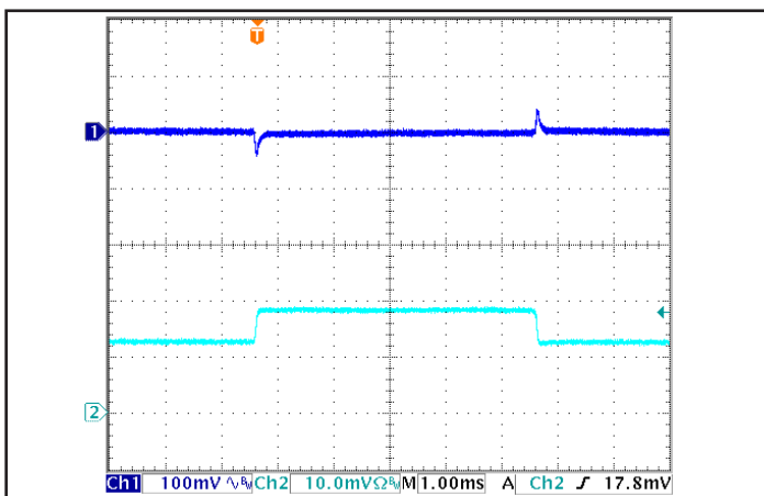
Figure 11: Output voltage response to step-change in load current (50%-75%-50% of I_{out(max)} ; dI/dt = 0.1A/\mu s ). Load cap: 100 \mu F electrolytic output capacitance. Top trace: V_{out} (100mV/div). Bottom trace: I_{out} (10A/div).
