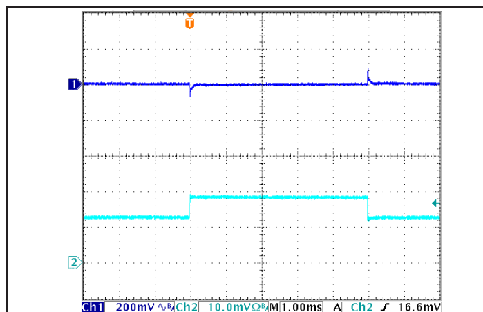
Figure 12: Output voltage response to step-change in load current (50%-75%-50% of I_{out(max)} ; dI/dt = 2A/\mu s ). Load cap: 330 \mu F electrolytic output capacitance. Top trace: V_{out} (200mV/div). Bottom trace: I_{out} (10A/div).
