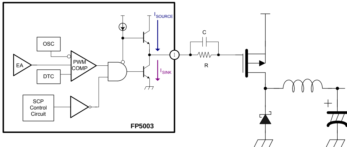
Figure 18. MOSFET Output Driving Cricuit
