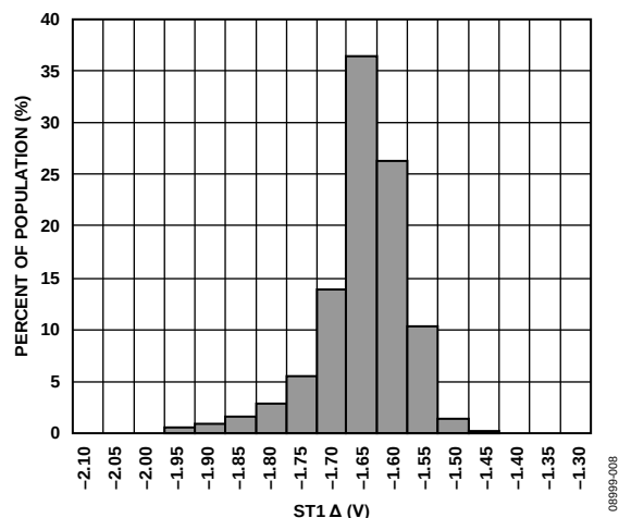
Figure 8. ST1 Output Change at 25°C ( V_{RATIO} = 5 V )
