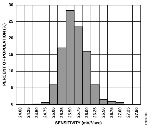
Figure 6. Sensitivity at 25°C ( V_{RATIO} = 5 V )
