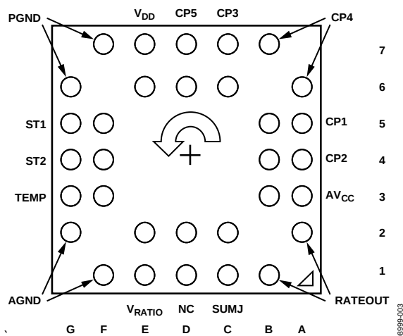
Figure 3. Pin Configuration
