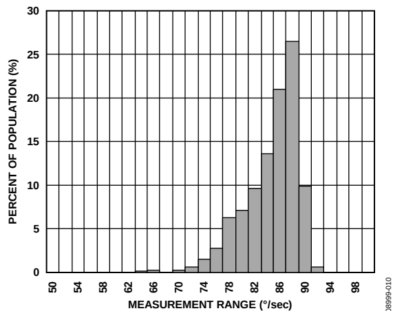
Figure 10. Measurement Range
