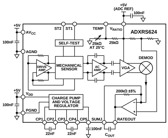
Figure 1. ADXRS624 Block Diagram
