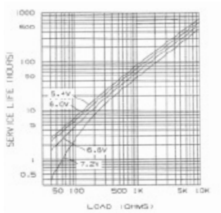
Typical Discharge Characteristics with Constant Resistance at 20°C
