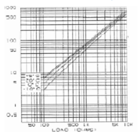
Typical Temperature Characteristics 5.4 Volts Cutoff Voltage
