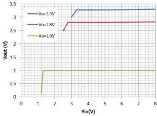
Line Regulation ( I_{out}=0mA )
