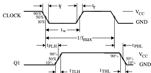
Figure 1. Switching Waveforms
