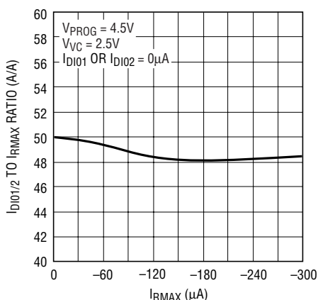
I_{DIO1/2} to I_{RMAX} Ratio vs R_{MAX} Current with a Lamp Fault
