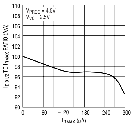
I_{DIO1/2} to I_{RMAX} Ratio vs R_{MAX} Current
