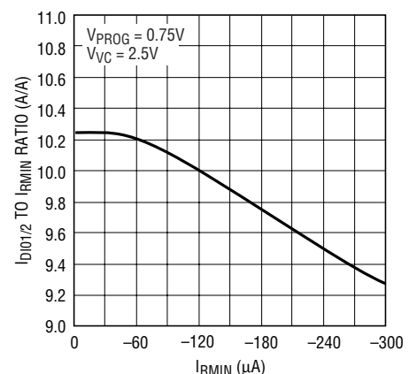
I_{DIO1/2} to I_{RMIN} Ratio vs R_{MIN} Current
