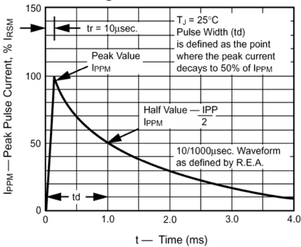
Fig. 3 – Pulse Waveform
