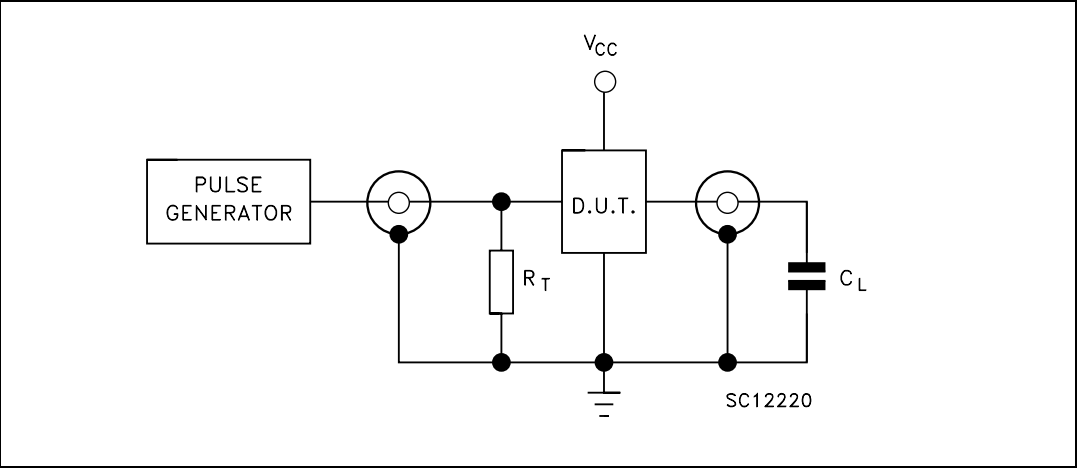
Figure 3. Test circuit
