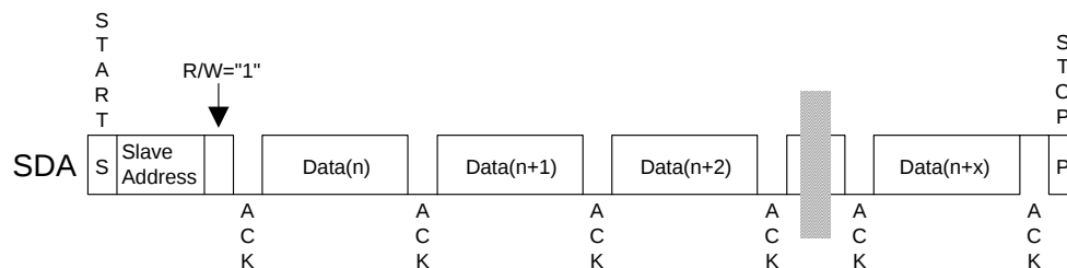
Figure 43. CURRENT ADDRESS READ
