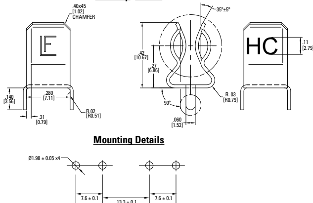
THT Clip-124061
