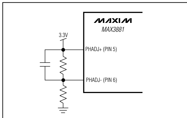
Figure 4. Phase-Adjust Resistor-Divider
