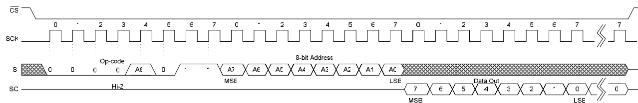
Figure 10. Memory Read
