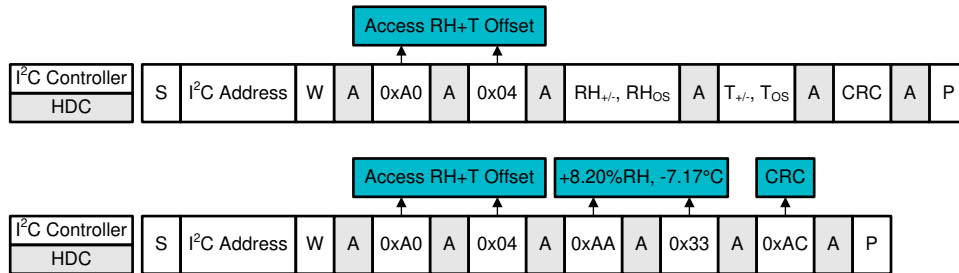
Figure 7-31. I 2 C Command Sequence: RH and T Offset (Example With +8.20% RH and -7.17^{\circ}C )
