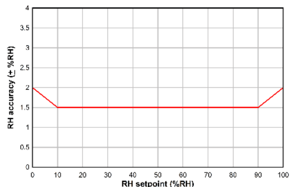
Typical RH Accuracy vs. RH Setpoint (T A = 25°C)
