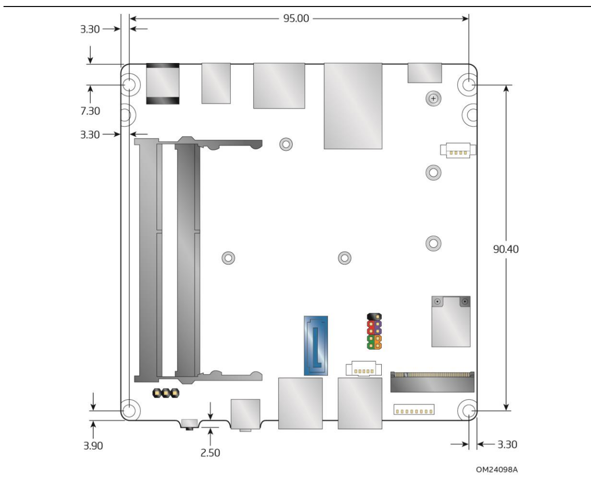
Figure 16. Board Dimensions
