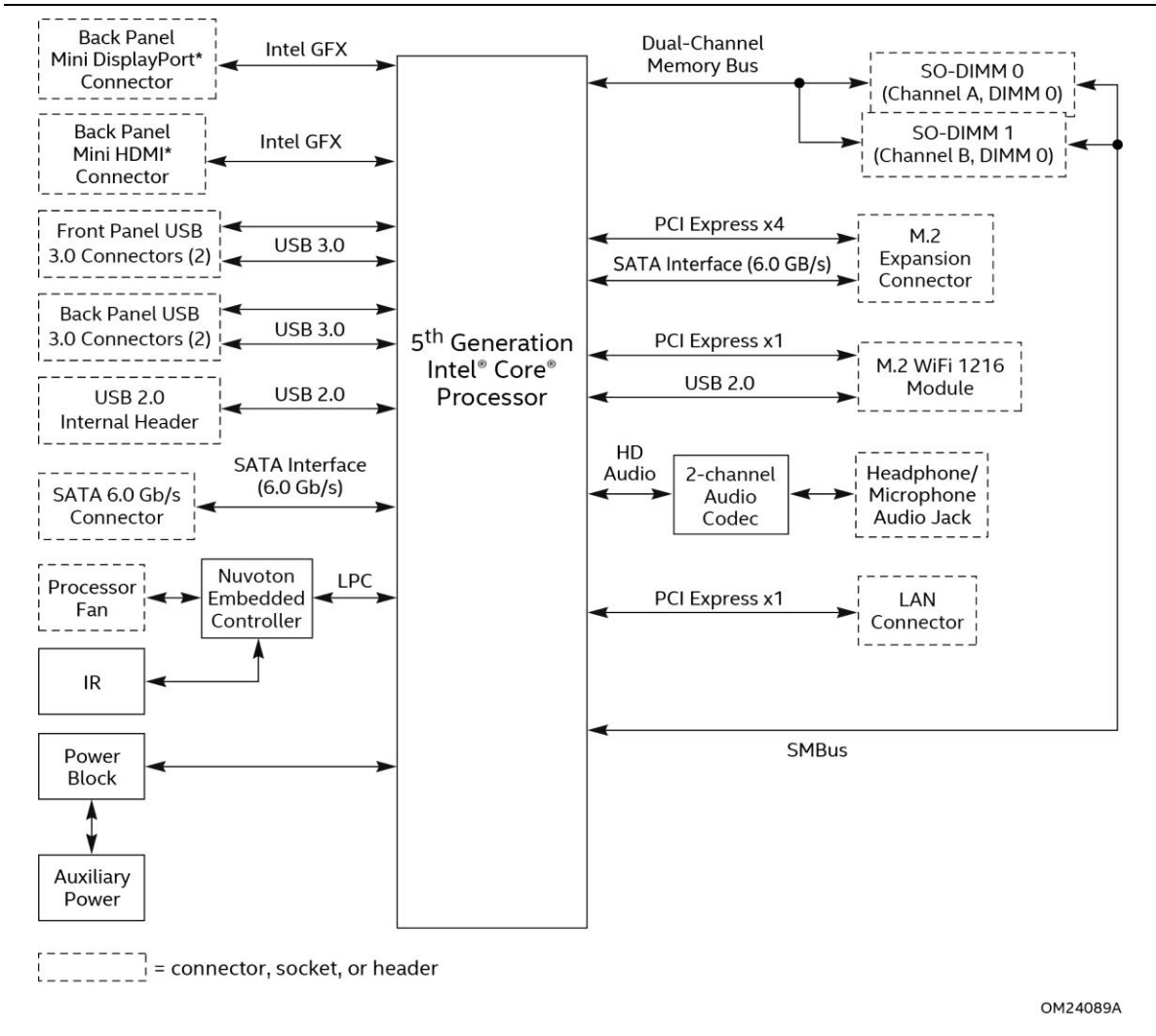
Figure 3. Block Diagram
