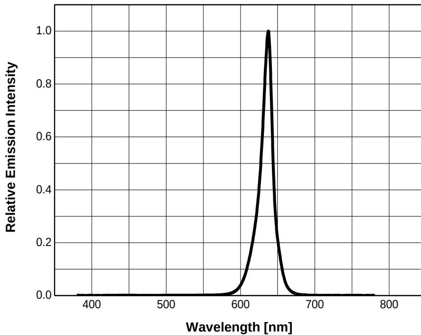
Fig 1. Color Spectrum, I_F = 20\text{mA} , T_j = 25^\circ\text{C} , RH30%
