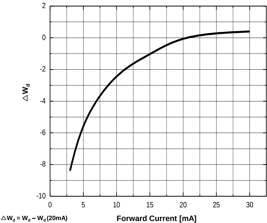
Fig 5. Forward Current vs. W_d Shift, T_j = 25^{\circ}\text{C}
