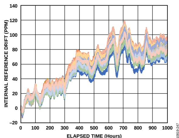
Figure 47. Reference Drift Through to 1000 Hours
