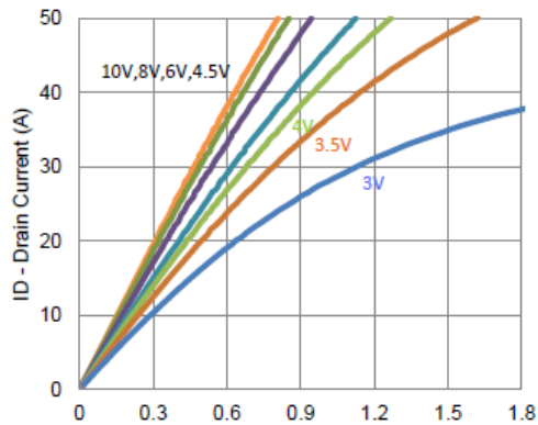
5. Output Characteristics
