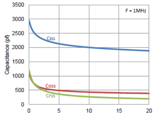
6. Capacitance
