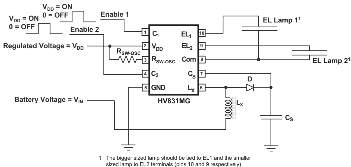
Figure 2: Split Supply Configuration
