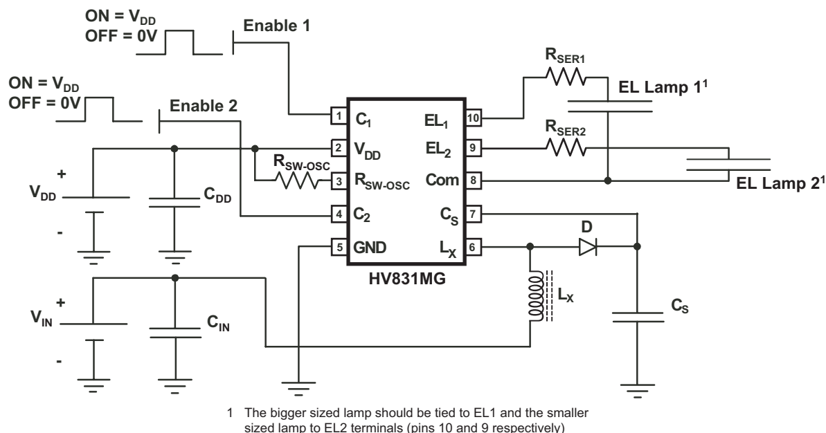
Figure 3: Typical Application Circuit For Audible Noise Reduction
