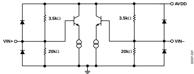
Figure 7. Analog Inputs
