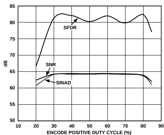
Figure 32. SINAD and SFDR vs. Clock Pulse Width High ( A_{IN} = 10.3 \text{ MHz} @ -0.5 \text{ dBFS} , 170 MSPS, LVDS)
