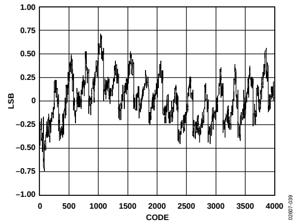
Figure 39. Typical INL Plot ( A_{IN} = 10.3 MHz @ -0.5 dBFS, 170 MSPS, LVDS)
