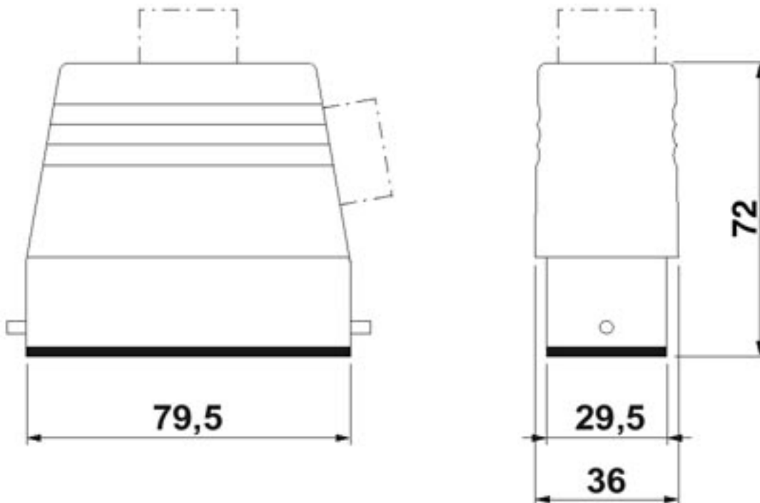
Dimensioned drawing
