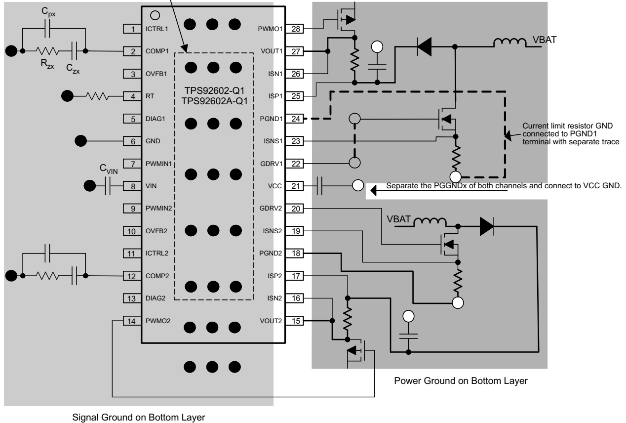
Figure 27. TPS92602-Q1 Board Layout
