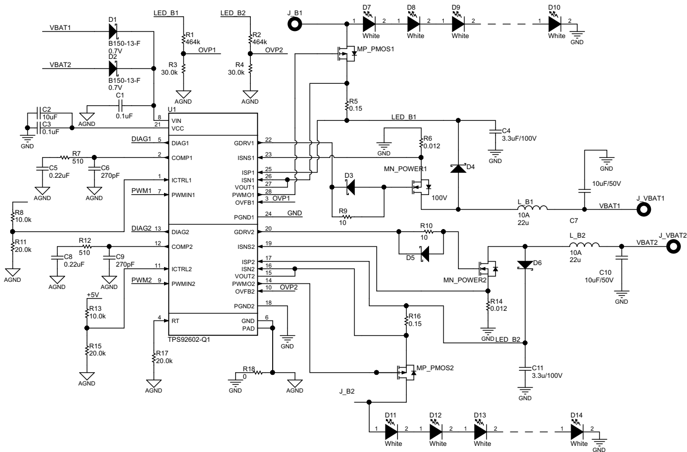
Figure 16. Boost Regulator ( V_{IN} < V_O ) Detailed Schematic
