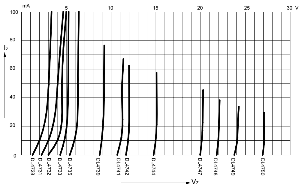
FIG.1 – BREAKDOWN CHARACTERISTICS
