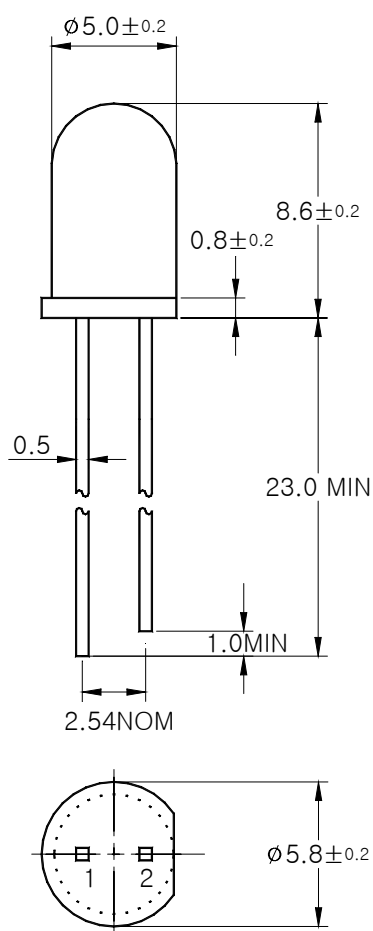
STRAIGHT TYPE
