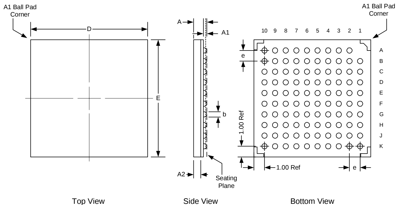
Figure 7. 99-Ball Grid Array (BGA)
