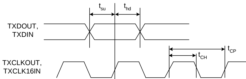
Figure 2. Data to Clock Delay
