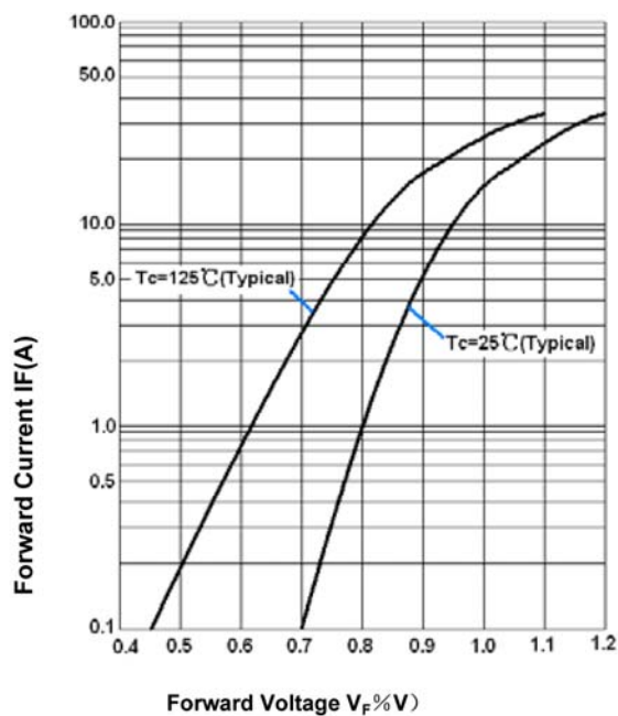
Fig.4 Forward Voltage
