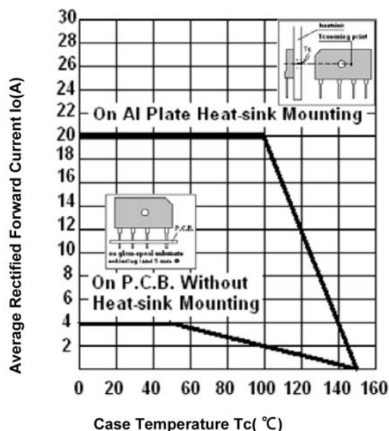
Fig. 1 derating Curve
