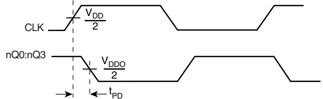
PROPAGATION DELAY
