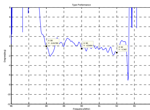
Phase Linearity(f0±2MHz)
