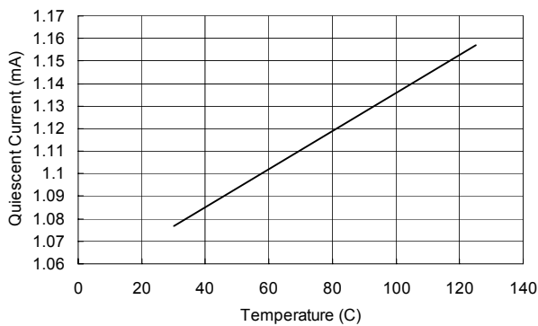
Quiescent Current vs Temperature (Output Voltage @ 2.5V)
