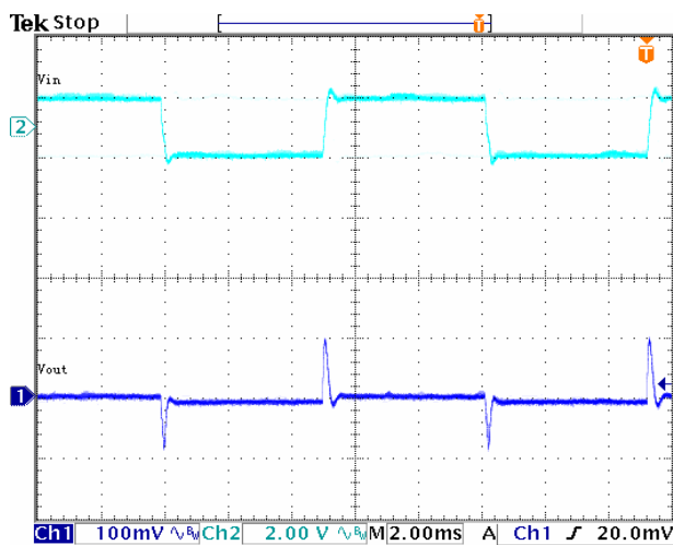
Line Transient
