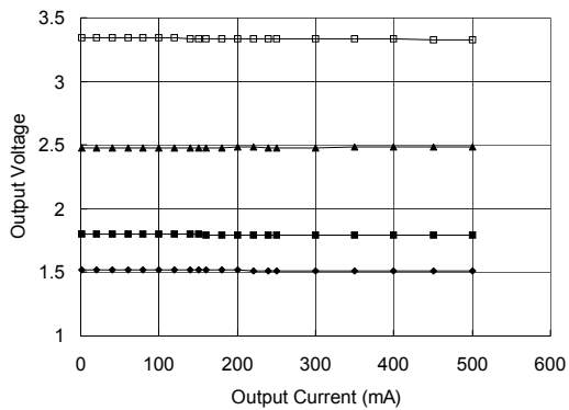
Load Regulation
