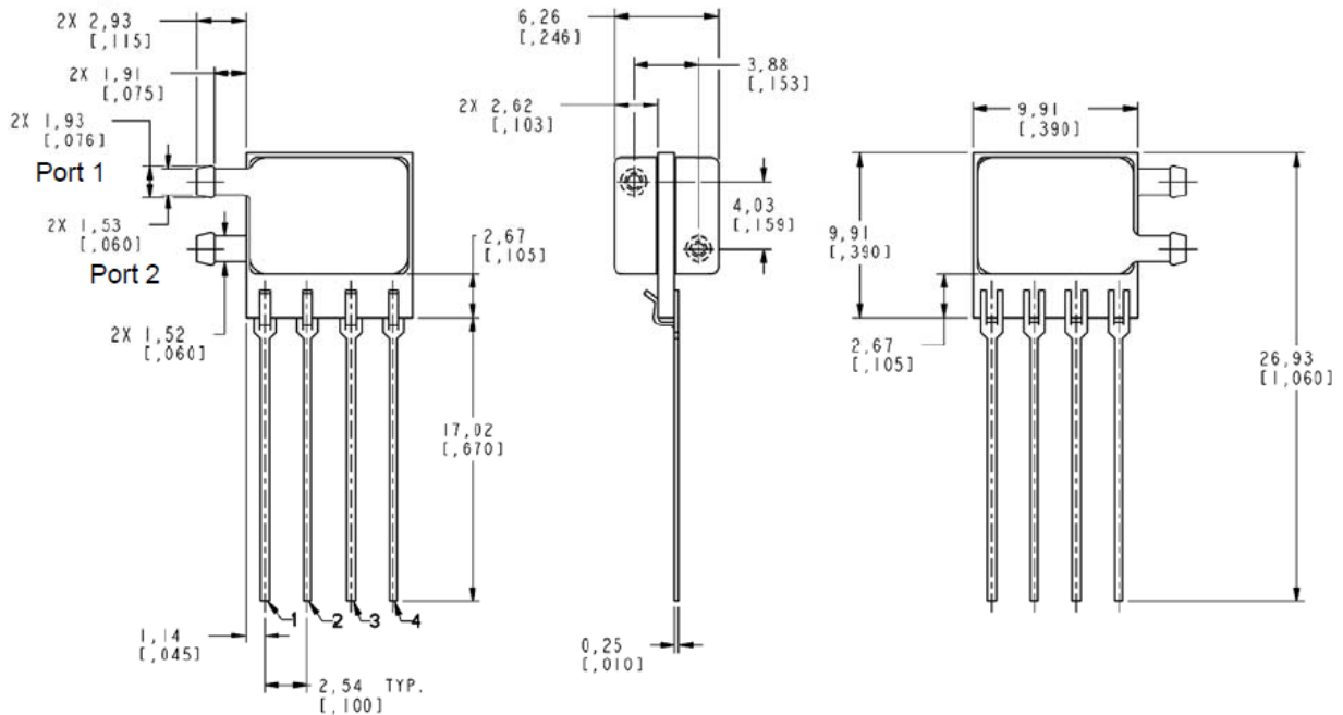
Figure 4. Package Dimensional Drawings (continued)
