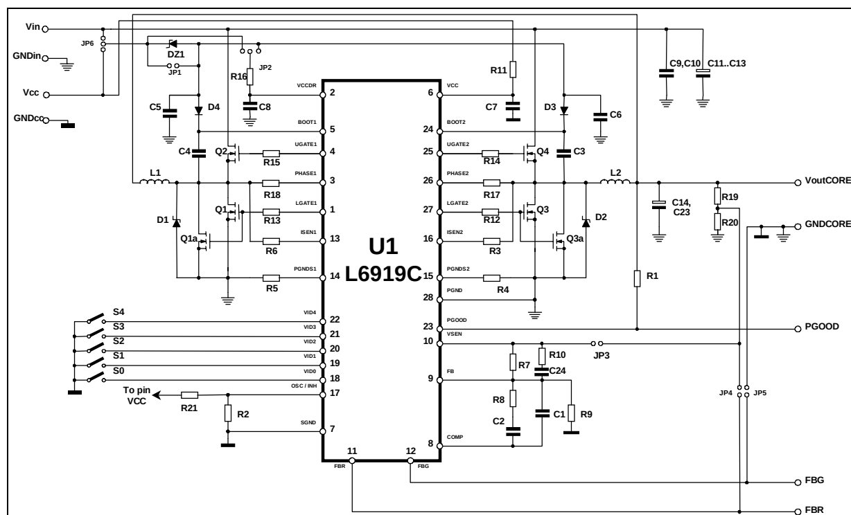
Figure 18. Demo Board Schematic
