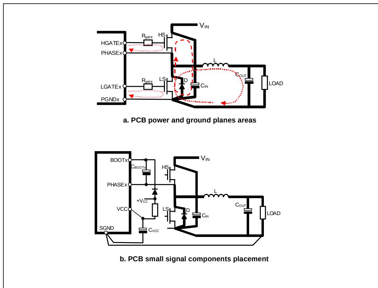
Figure 15. Power connections and related connections layout guidelines (same for both phases)
