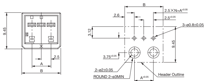
PC Board Layout Acceptable Board Thickness : 1.6±0.3
