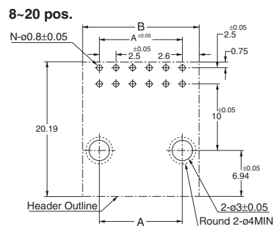
Acceptable Board Thickness : 1.6 \pm 0.3
