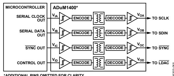
Figure 37. Isolated Interface
