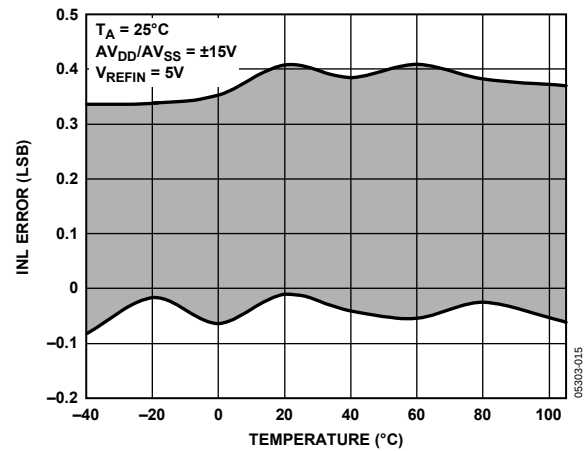
Figure 11. Integral Nonlinearity Error vs. Temperature, AV_{DD}/AV_{SS} = \pm 15\text{ V}
