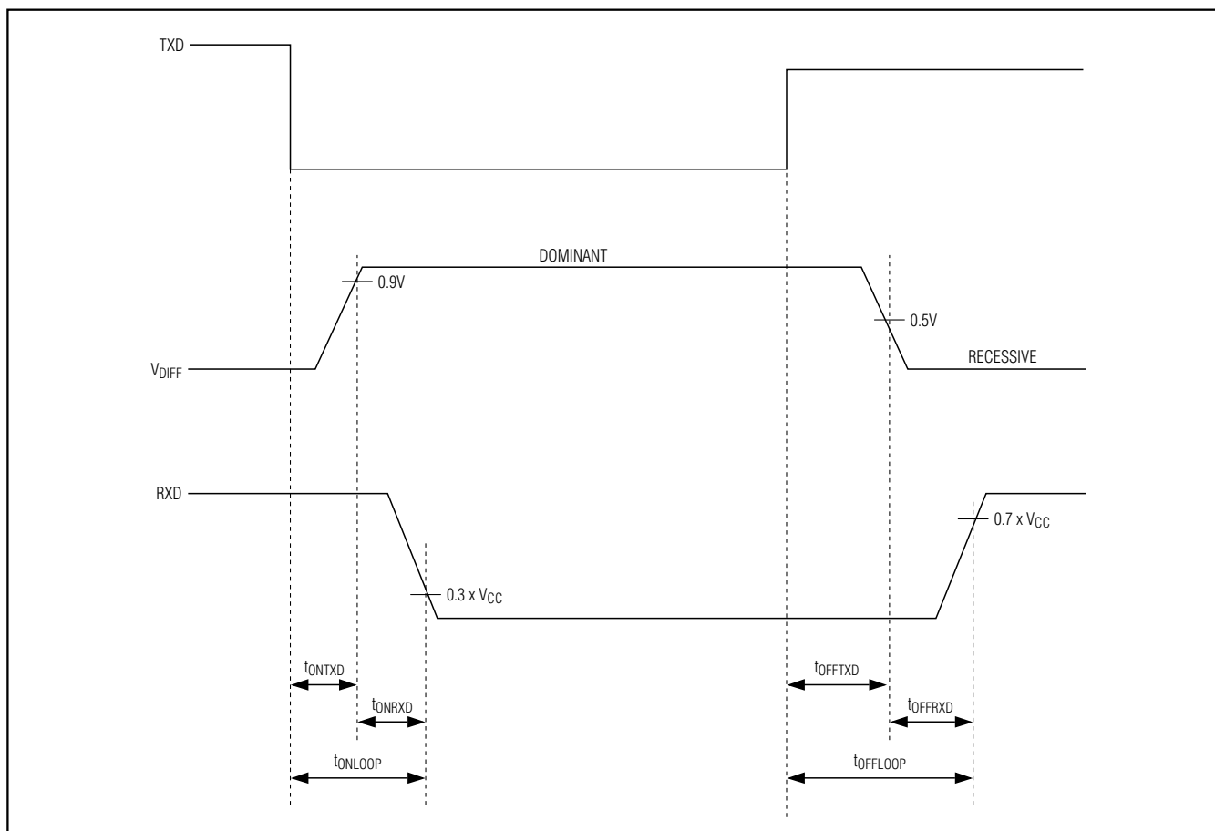
Figure 1. Timing Diagram
