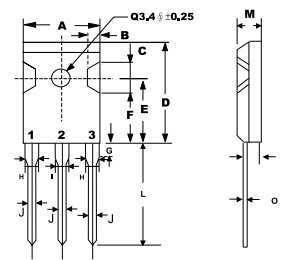
TO-247 (3P)
