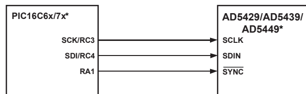
Figure 54. PIC16C6x/7x-to-AD5429/AD5439/AD5449 Interface
