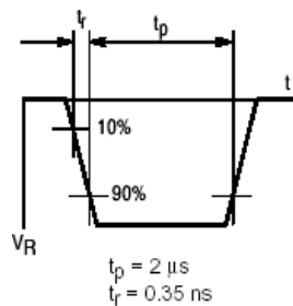
INPUT PULSE
