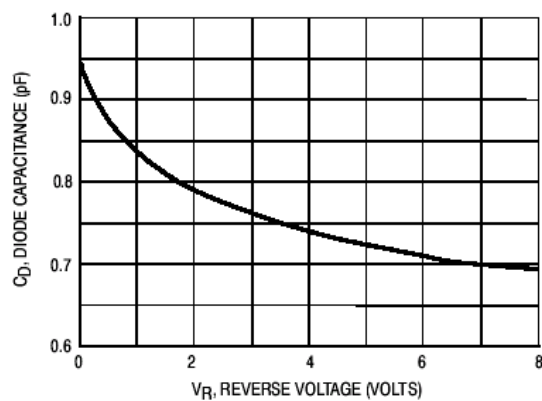
Figure 3. Diode Capacitance
