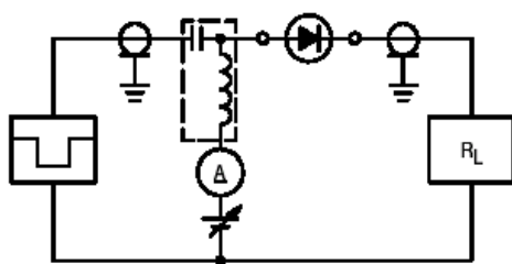
RECOVERY TIME EQUIVALENT TEST CIRCUIT
