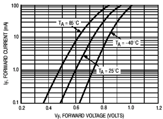
Figure 1. Forward Voltage
