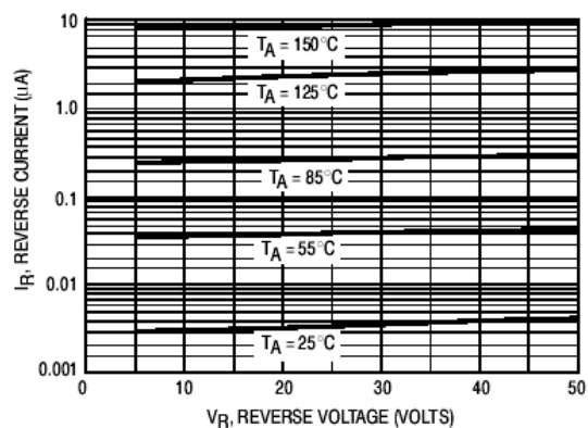
Figure 2. Reverse Current
