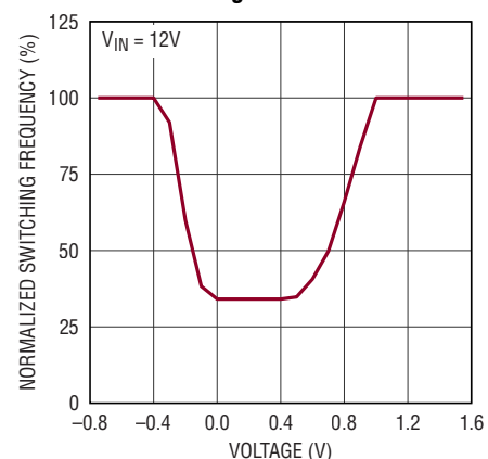
Normalized Switching Frequency vs FBX Voltage
