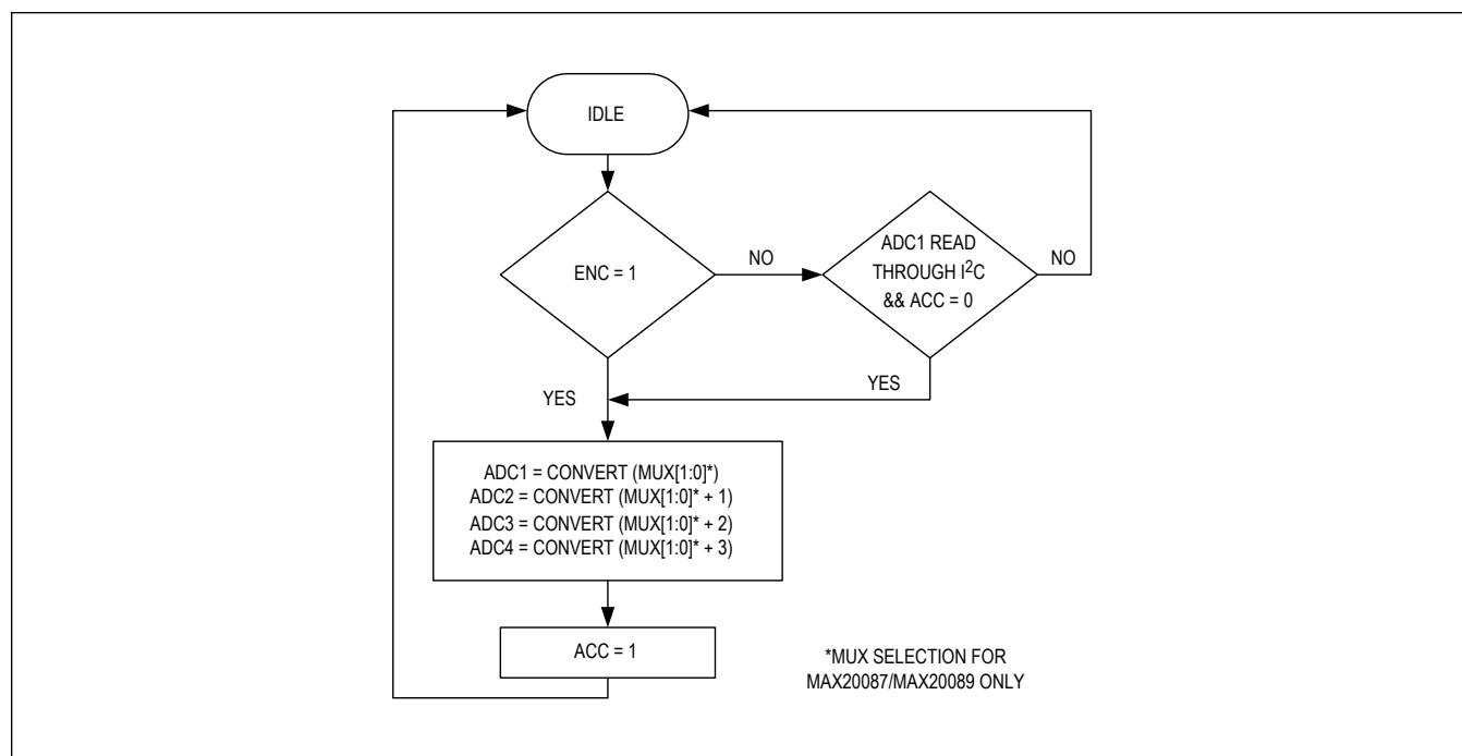
Figure 5. ADC Flow Diagram
