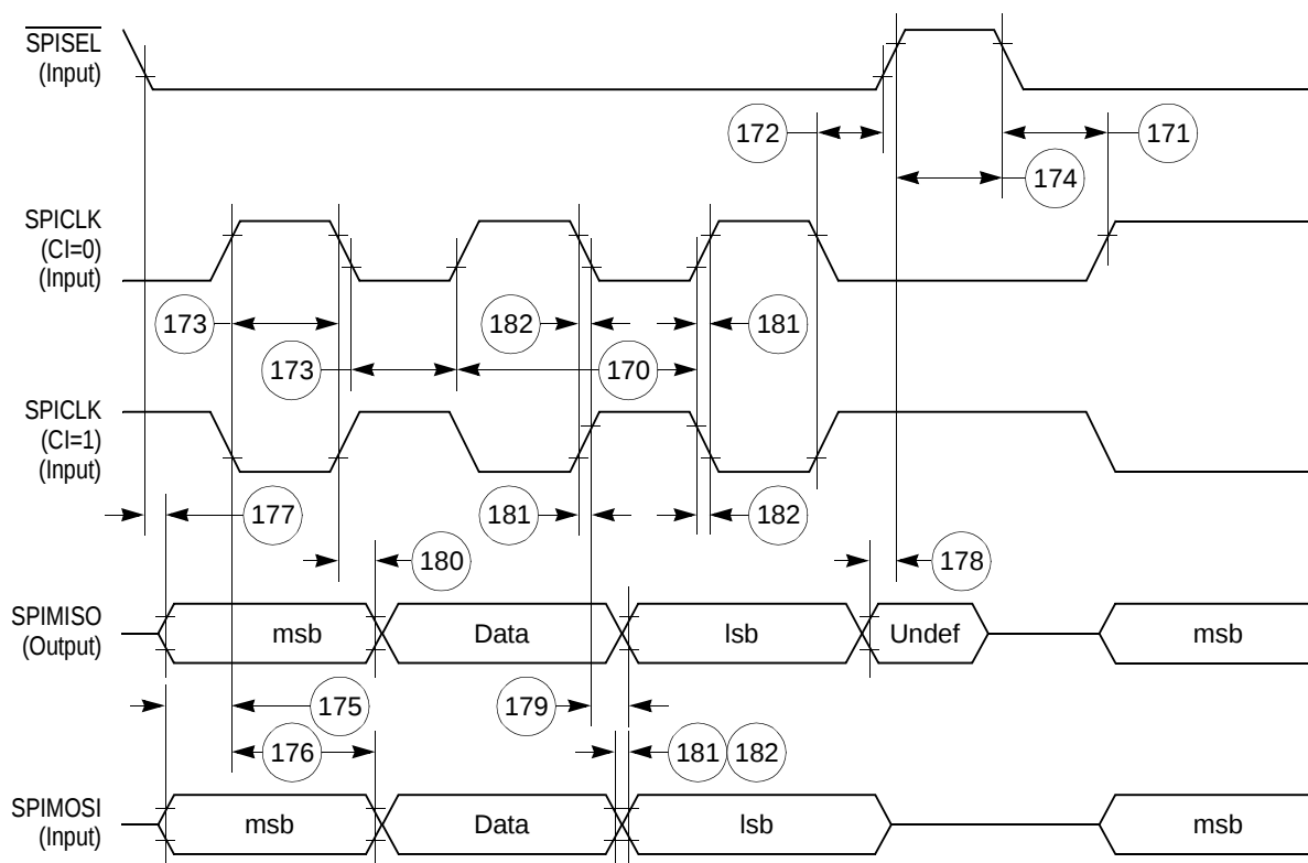
Figure 67. SPI Slave (CP = 0) Timing Diagram
